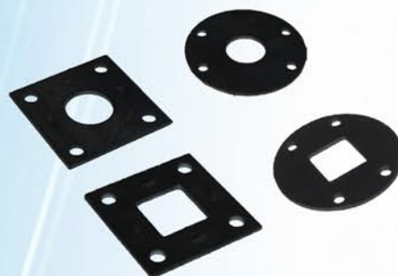
Mounting Plates JS-MP39RE st. 39 Round Axle (Electric Brake) JS-MP39RH st. 39 Round Axle (Hydraulic Brake) JS-MP40SE st. 40 Square Axle (Electric Brake) JS-MP40SH st. 40 Square Axle (Hydraulic Brake)
