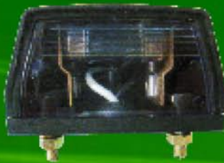
JS-NPLG-67 Number Plate light Globe
