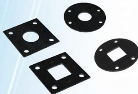
Mounting Plates JS-MP39RE st. 39 Round Axle (Electric Brake) JS-MP39RH st. 39 Round Axle (Hydraulic Brake) JS-MP40SE st. 40 Square Axle (Electric Brake) JS-MP40SH st. 40 Square Axle (Hydraulic Brake)
